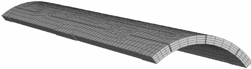
Figure 2 Section of basepipe with C3D8R mesh
