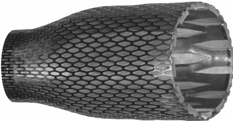
Figure 4 Example of partially expanded ESS
