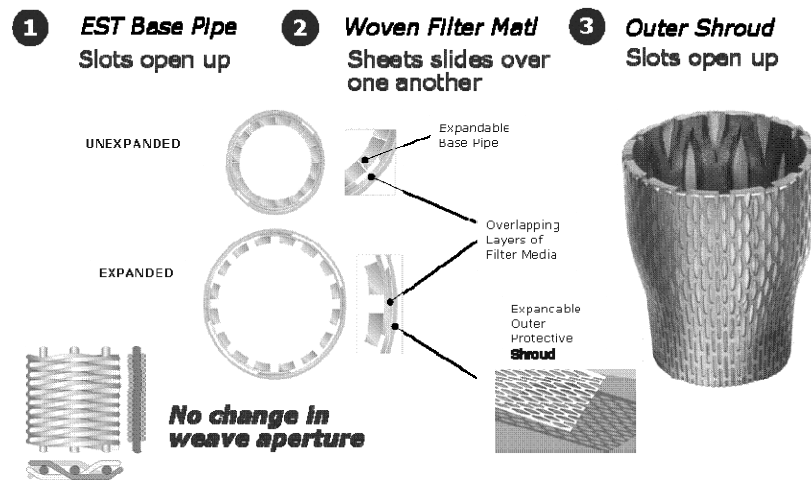
Figure 1 Details of the construction of the ESS
