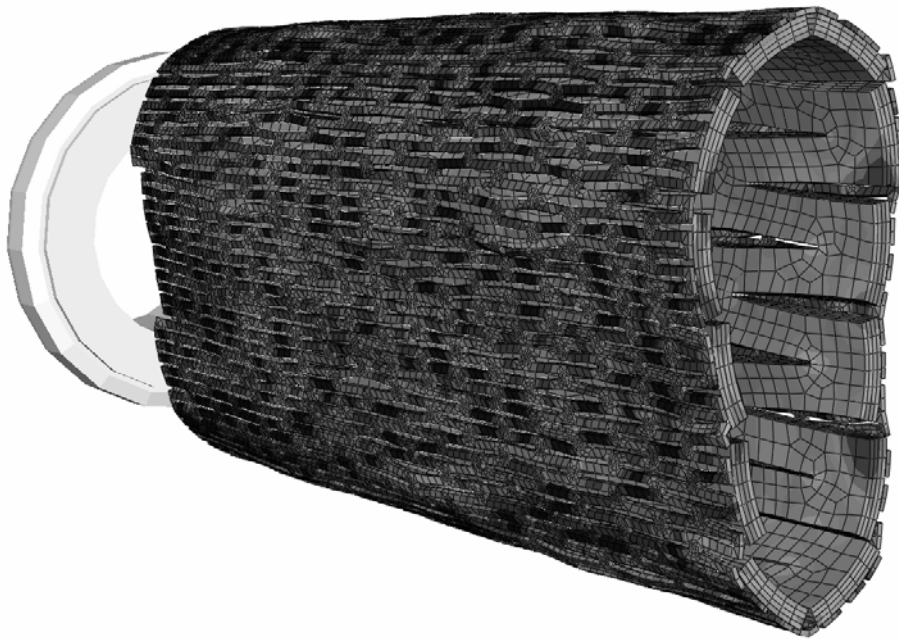
Figure 5 Hydraulically collapsed ESS sample
