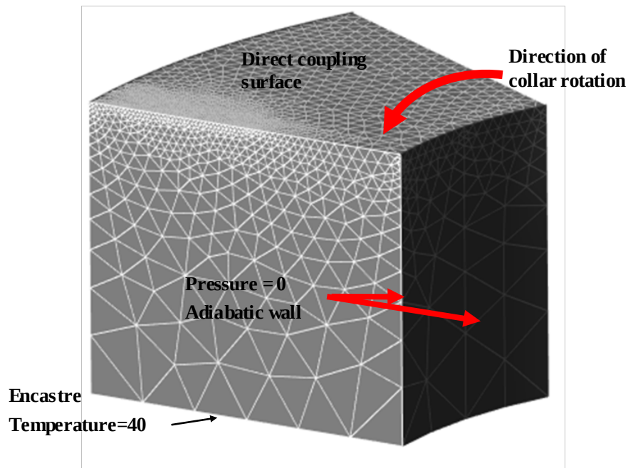
Figure 2. Finite-element model of shoe.
