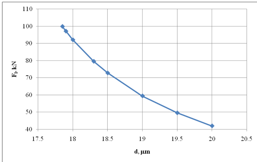
Figure 4. Dependence of lift force in thrust bearing on initial clearance value.
