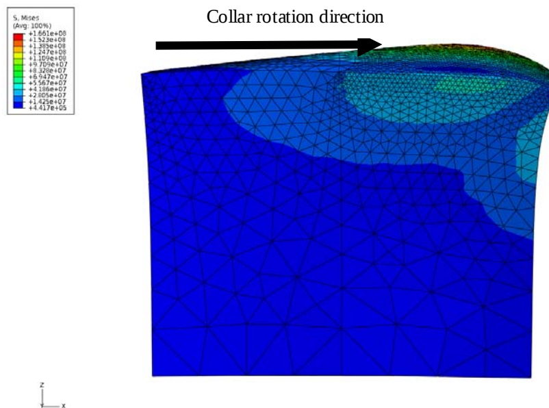
Figure 8. Distribution of stress in shoe.
