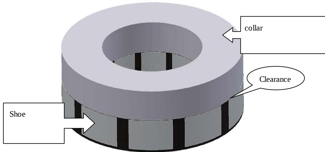
Figure 1. Design of thrust bearing.
