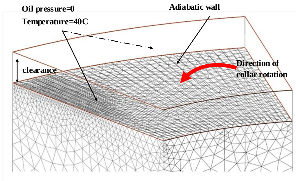
Figure 3. Oil flow computational domain.
