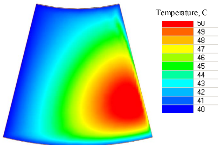
Figure 6. Distribution of temperature in clearance for 80 tons rotor.
