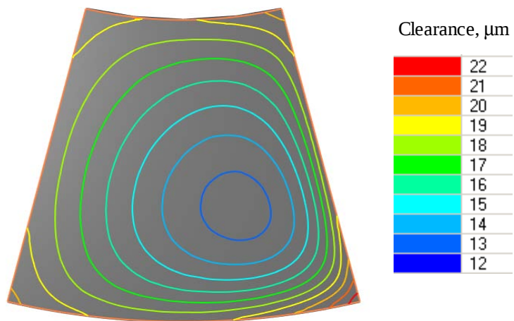
Figure 5. Distribution of distance between shoe and collar for 80 tons rotor.
