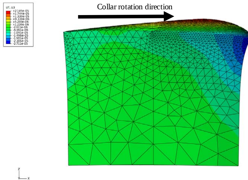
Figure 7. Displacement of shoe material along z axis. Deformation is magnified in 1000 times.
