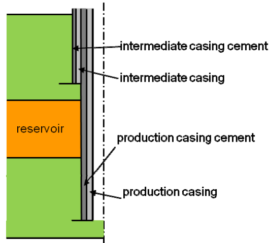
Figure 1. Typical cased-hole well-system.
