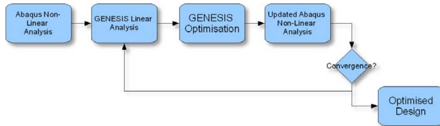
Figure 1. Coupled Optimisation Workflow.
