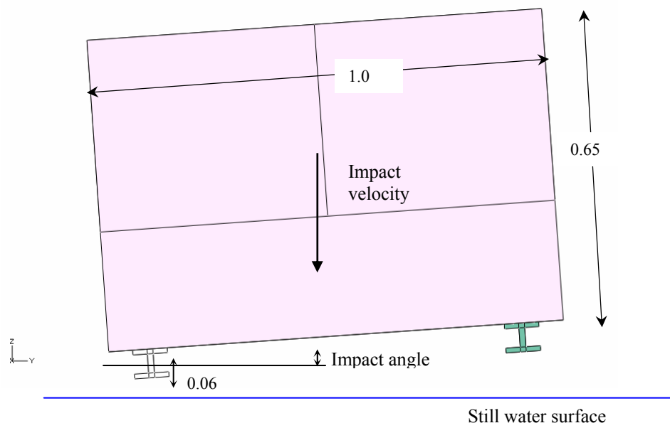
Figure 2: Drop test conditions
