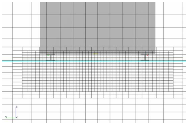
Figure 6: The CFD mesh with local adaptation near impact region
