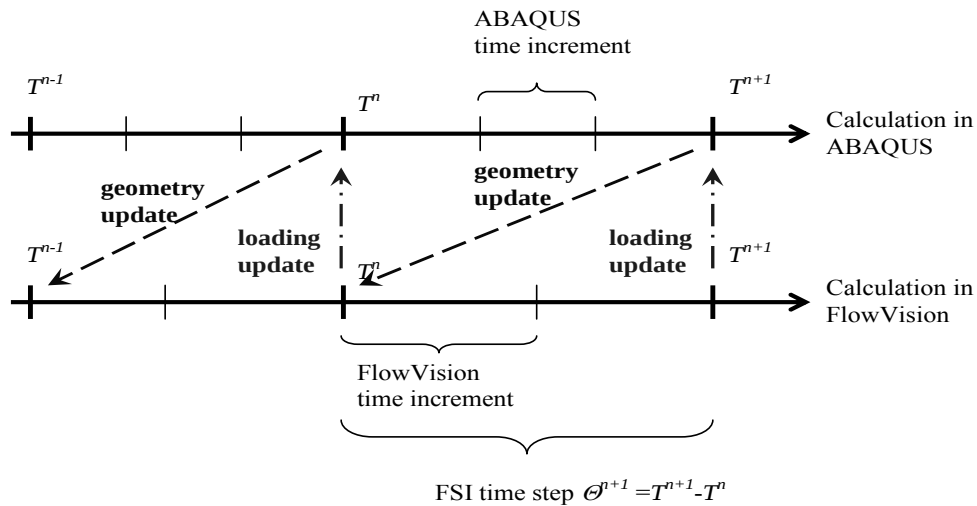
Figure 6.1: FSI time step for FlowVision and Abaqus
