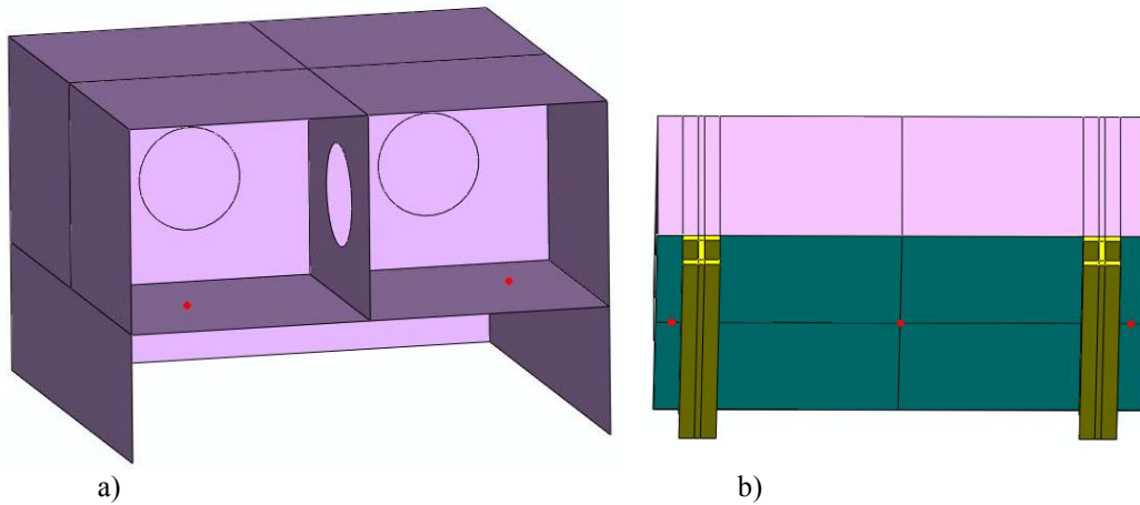
Figure 3: Location of points for values time history: a) on inner container structure (for strain values) b) on impact surface (for pressure values)
