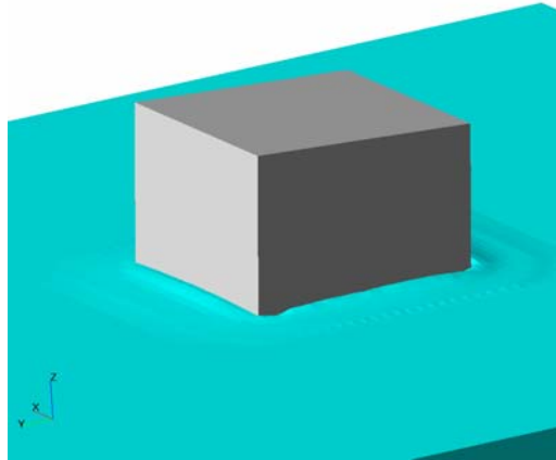
Figure 8: Free surface distribution after impact, 4 degree inclination of container
