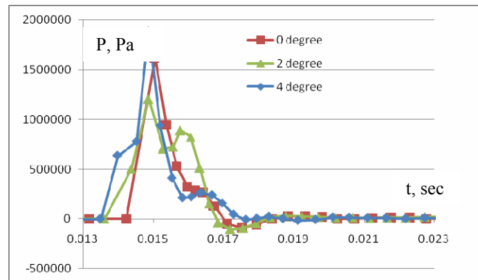
Figure 11: Dependence pressure on time at area of pressure sensor at the center of a bottom
