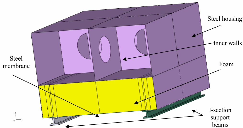
Figure 1: Components of testing drop-test structure
