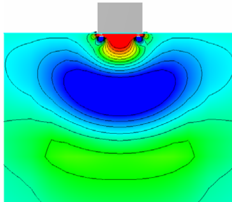
Figure 7: Acoustic wave after impact of the container with water, 0 degree inclination
