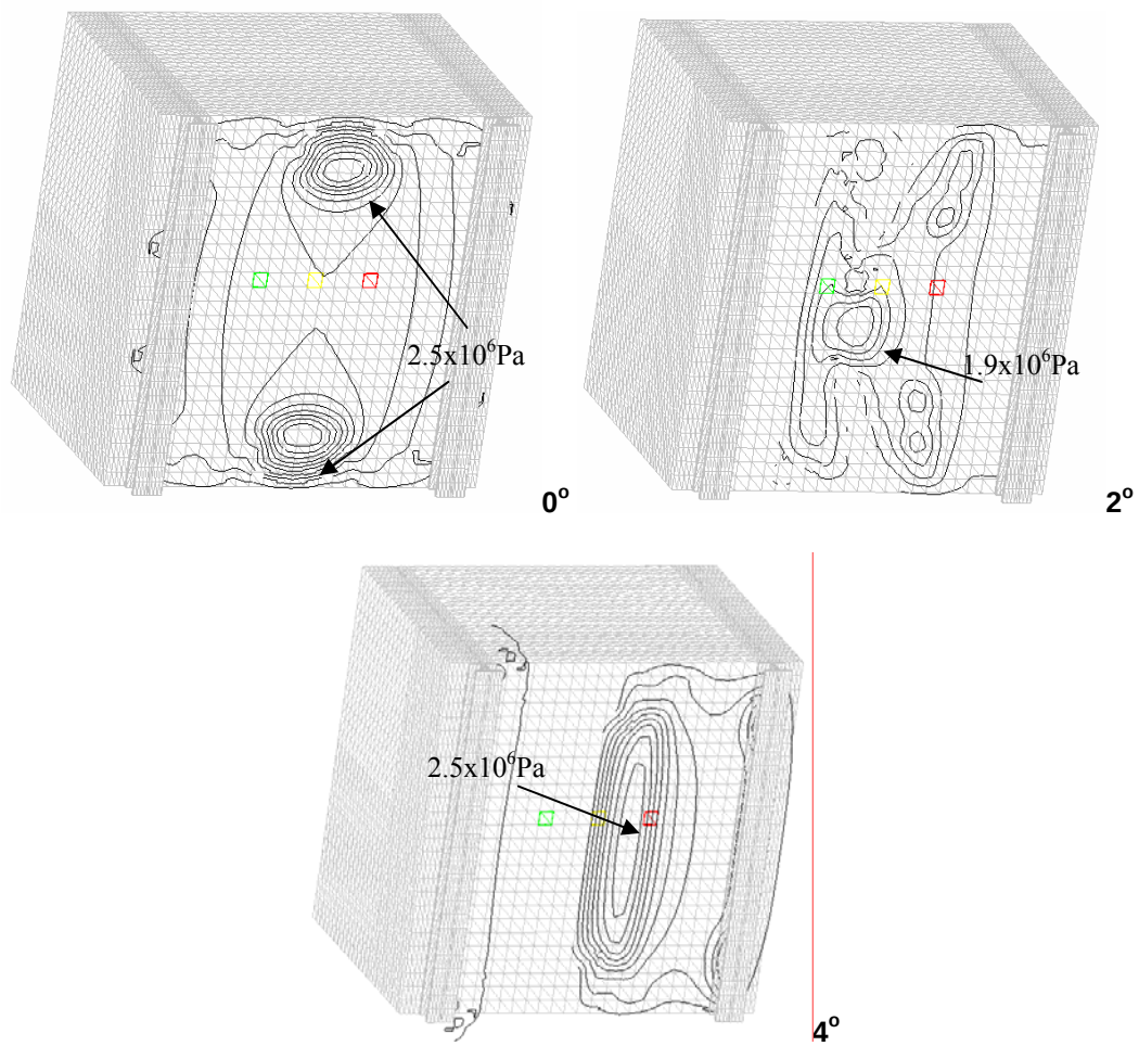
Figure 10: Pressure distribution in plane near bottom, t=0.015\text{s} after start motion, isolines step = 3 \times 10^5 \text{ Pa}
