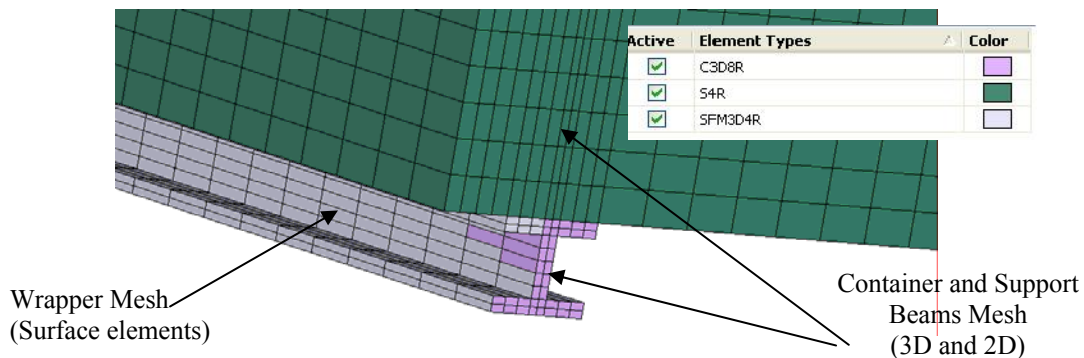
Figure 4: Wrapper mesh defined for the container surface
