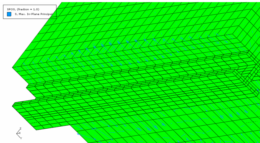
Figure 13: Maximum principal stress near junction of the container bottom membrane and container walls
