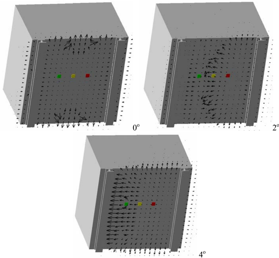
Figure 9: Velocity distribution in plane near bottom, t=0.015s after start motion.
