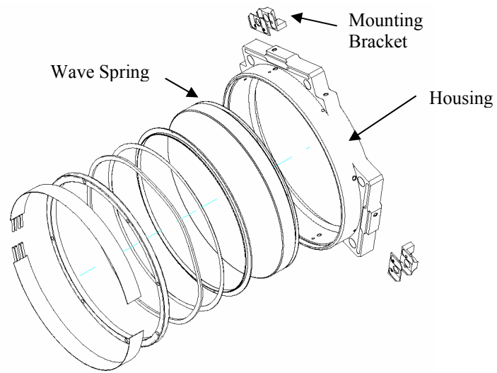
Figure 15. Optical lens assembly.
