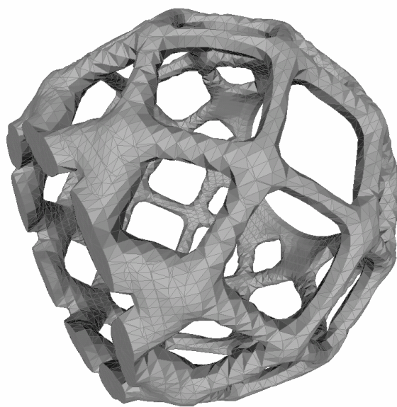
Figure 13. Pure torsion, infinite domain - numerically generated topology.
