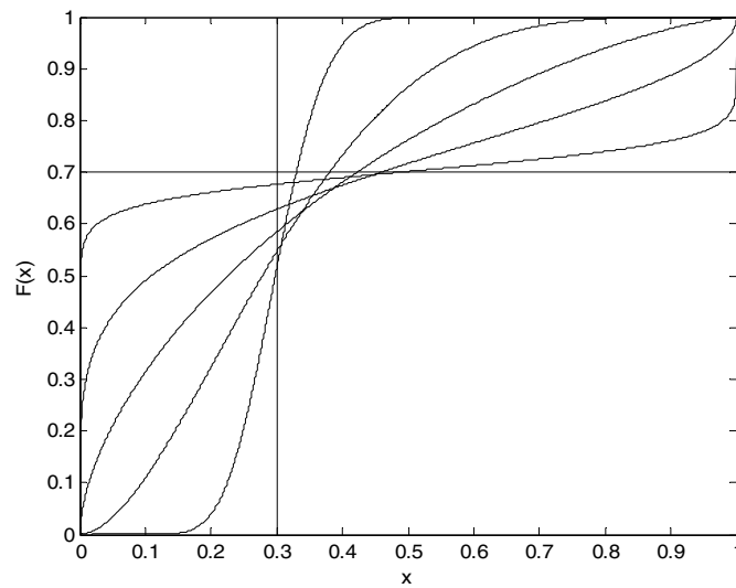
Figure 2. Transition from initial to final cumulative distribution for t=0.0, 0.1, 0.3, 0.5, 0.7, 0.9 and 1.0 .
