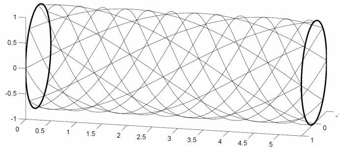
Figure 7. Helical spirals for combined axial and torsion loads ( \gamma=\pi/6 ).
