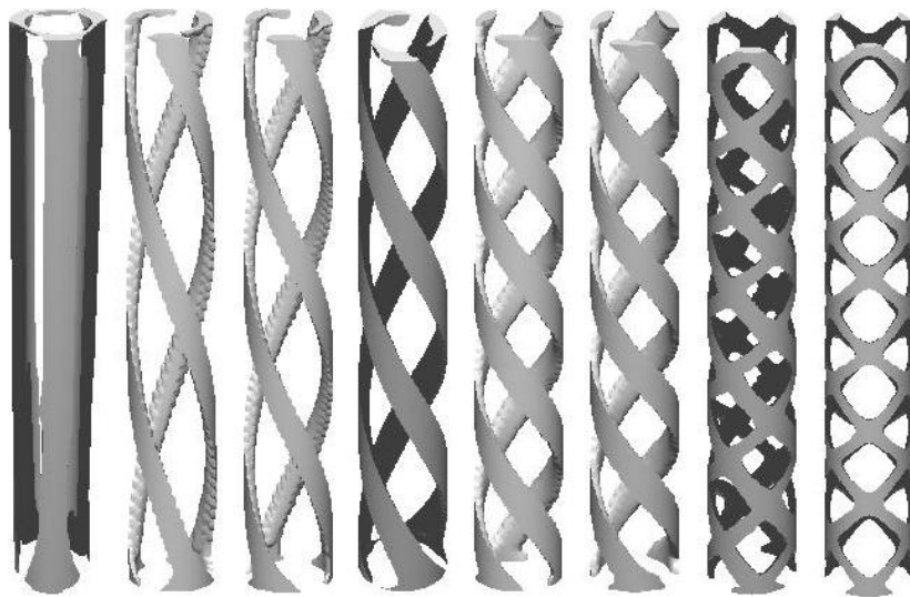
Figure 9. Results for combined axial and torsion loads ( f_n/f_t = \infty, 3.464, 2.383, 1.678, 0.727, 0.352 and 0 )
