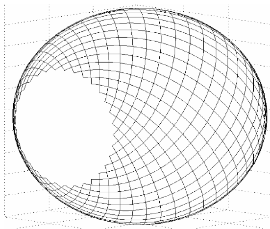
Figure 12. Michell's loxodrome for pure torsion.
