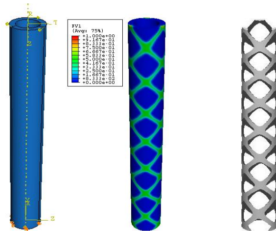
Figure 8. Pure torsion, cylindrical domain – numerically generated topology.
