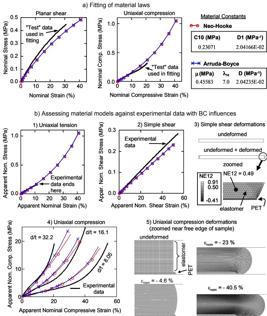
Figure 5: Results of fitting “corrected” material data and then assessing the validity of the resulting material models by simulating the original tests including the influence of the test’s boundary conditions.
