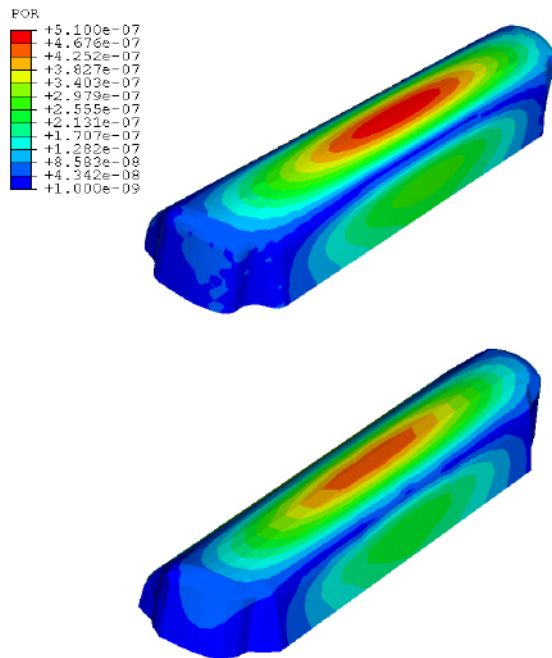
Figure 5: Comparison of acoustic pressures obtained from acoustic infinite element model (top) and the impedance model (bottom) for the prototype cover
