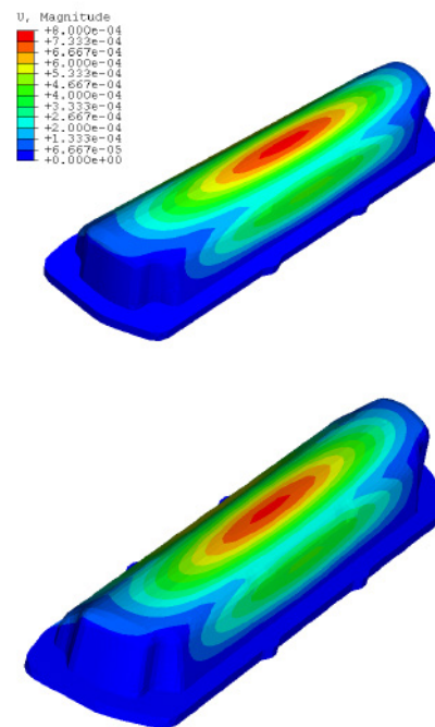
Figure 4: Comparison of surface displacements obtained from acoustic infinite element model (top) and the impedance model (bottom) for the prototype cover
