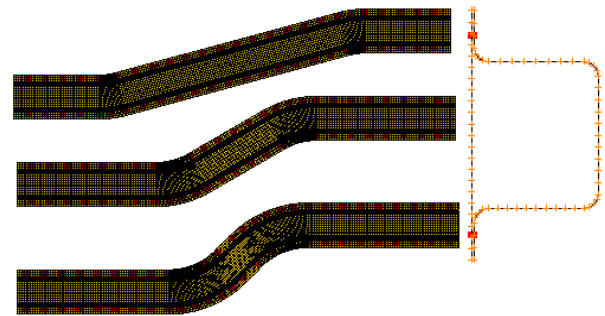
Figure 3: Undeformed model and cross-section for 15°, 30°, and 45° frames. Red dots represent spot weld locations.
