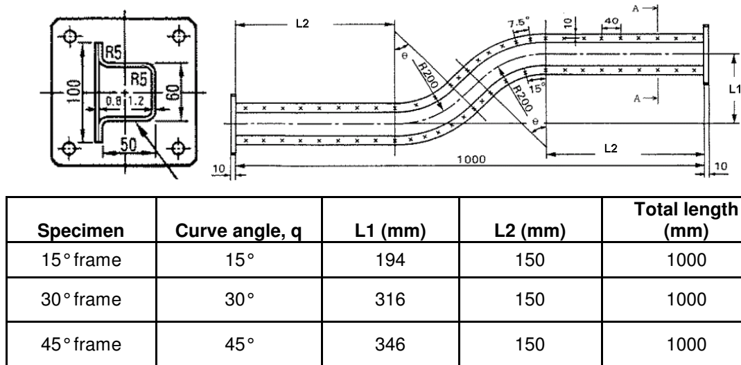
Figure 1: Profile and major dimensions of test specimen. Dots represent spot welds (Ref. 2).
