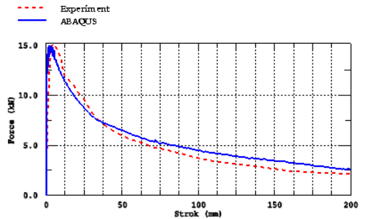
Figure 8: Load-displacement behavior of 45° frame.
