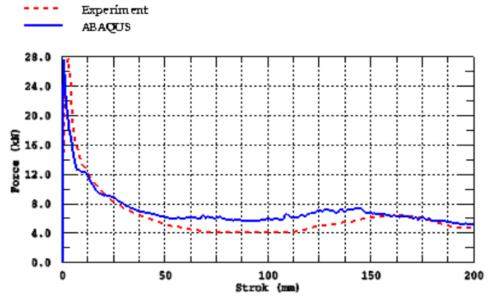
Figure 6: Load-displacement behavior of 15° frame.
