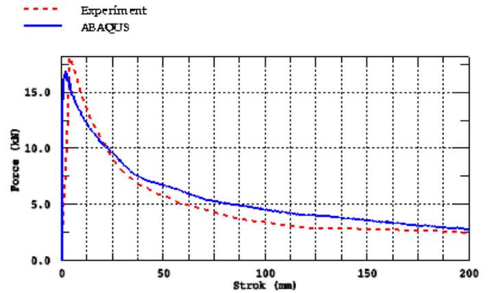
Figure 7: Load-displacement behavior of 30° frame.
