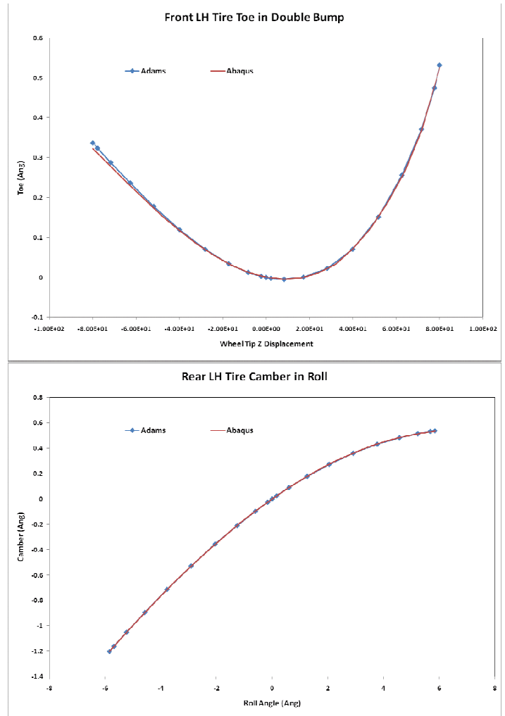
Figure 3: Representative parameters from kinematics simulation; toe in double bump test (top), camber in roll test (bottom)
