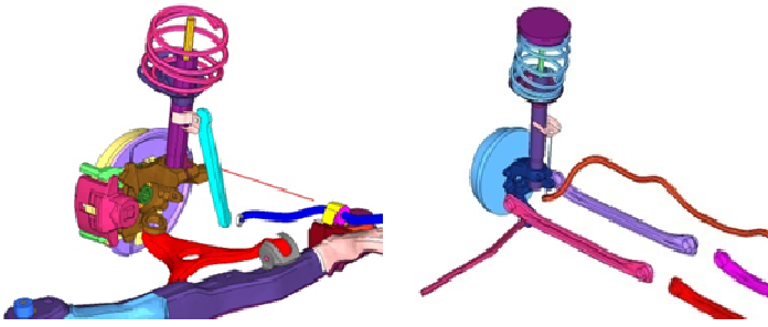
Figure 1: MacPherson strut front (l) and rear (r)
