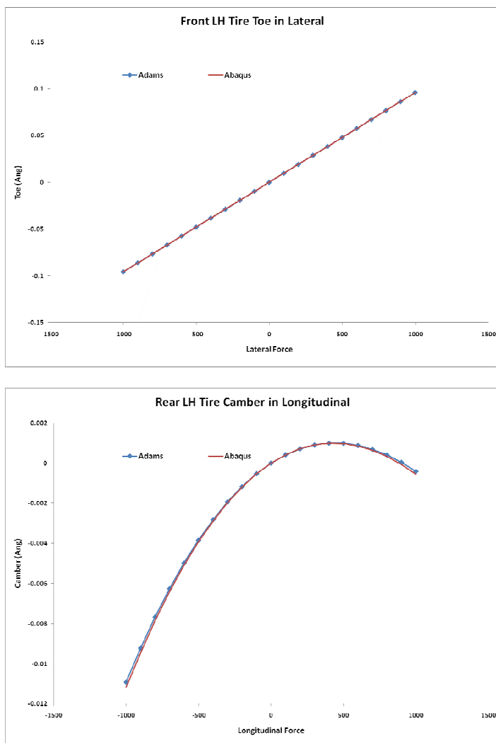
Figure 4: Representative parameters from compliance simulation; toe in lateral compliance (top) camber in longitudinal compliance (bottom)
