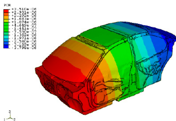
Figure 5: Air pressure distribution for the second acoustic eigenmode at 79.6 Hz.
