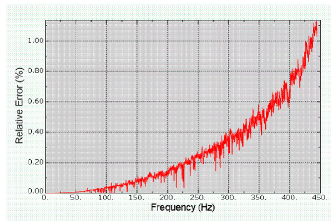
Figure 2: Relative error in natural frequencies obtained by Abaqus/AMS with respect to those obtained by the Lanczos eigensolver.
