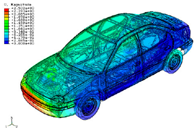
Figure 3: The 10th structural eigenmode at 6.6 Hz
