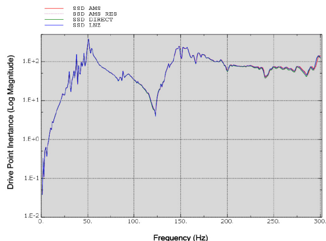
Figure 6: Point inertance at front left drive point.
