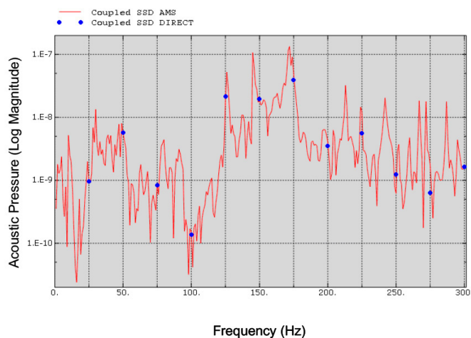
Figure 8: Acoustic pressure at the ear position.
