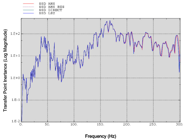
Figure 7: Transfer inertance at driver seat.
