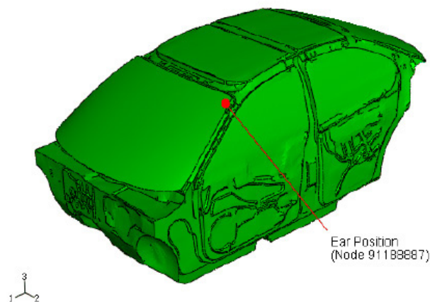
Figure 4: The air volume inside the vehicle.
