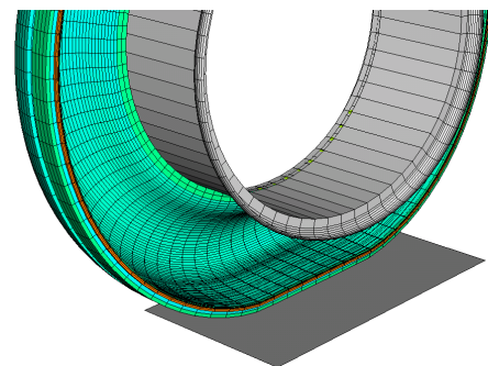
Figure 6: Partial three-dimensional model with footprint loading.
