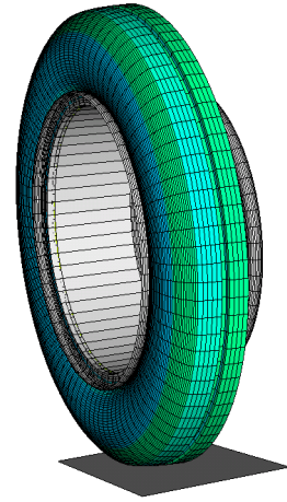
Figure 5: Partial three-dimensional model generated using symmetric model generation.
