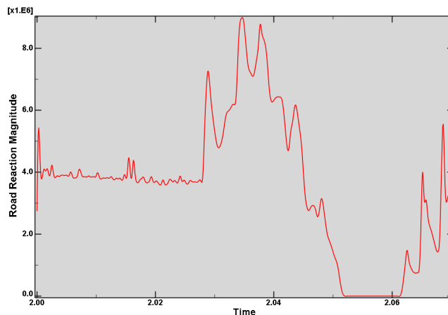
Figure 16: Vertical reaction force magnitude at road reference point.
