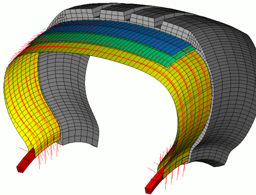
Figure 3: Reinforcement orientation in the belts and the carcass in three dimensions.
