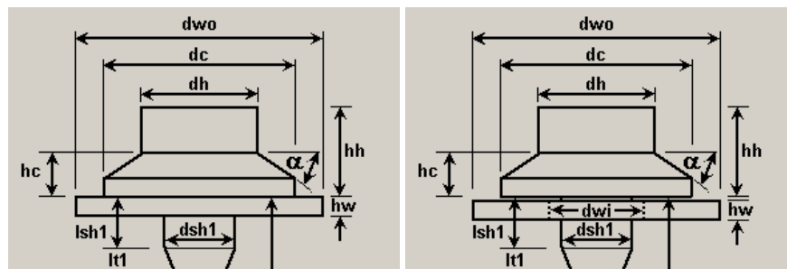
Figure 6. Washer types.
