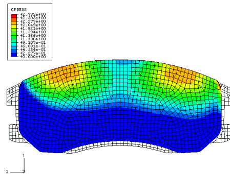
Figure 7a: Contact pressure distribution on the outboard lining at the end of Step 3
