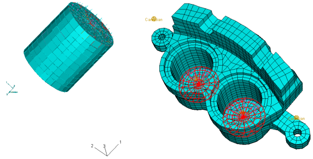
Figure 3: Caliper and piston, with pressure-loaded surfaces highlighted
