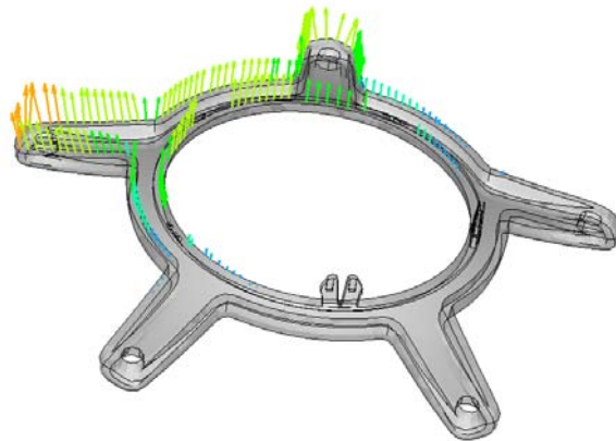
Figure 2. Example of penetration detection between two pieces.
