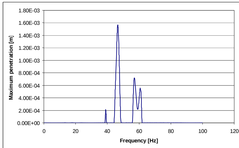
Figure 3. Example of the maximum detected penetration within the frequency range for all connectors
