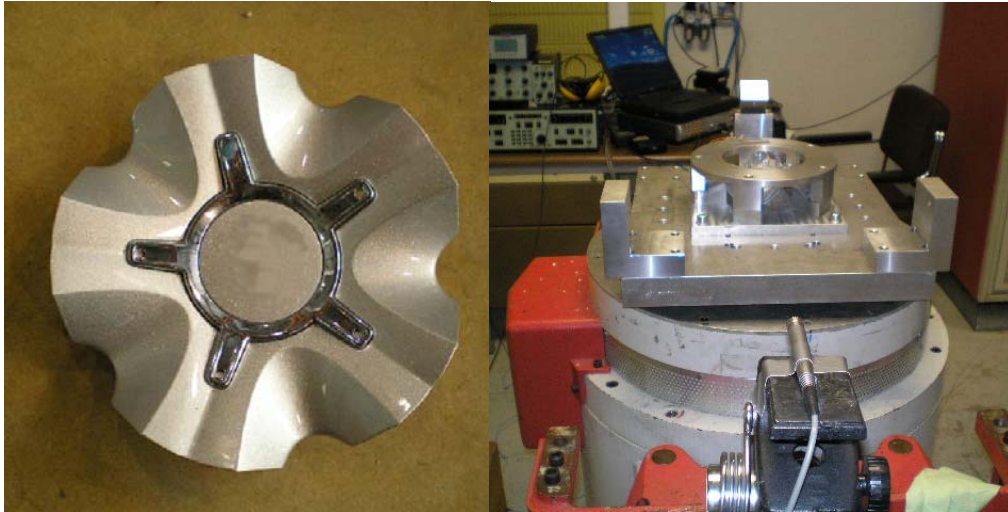
Figure 5. Wheel trim used for the study and testing layout
