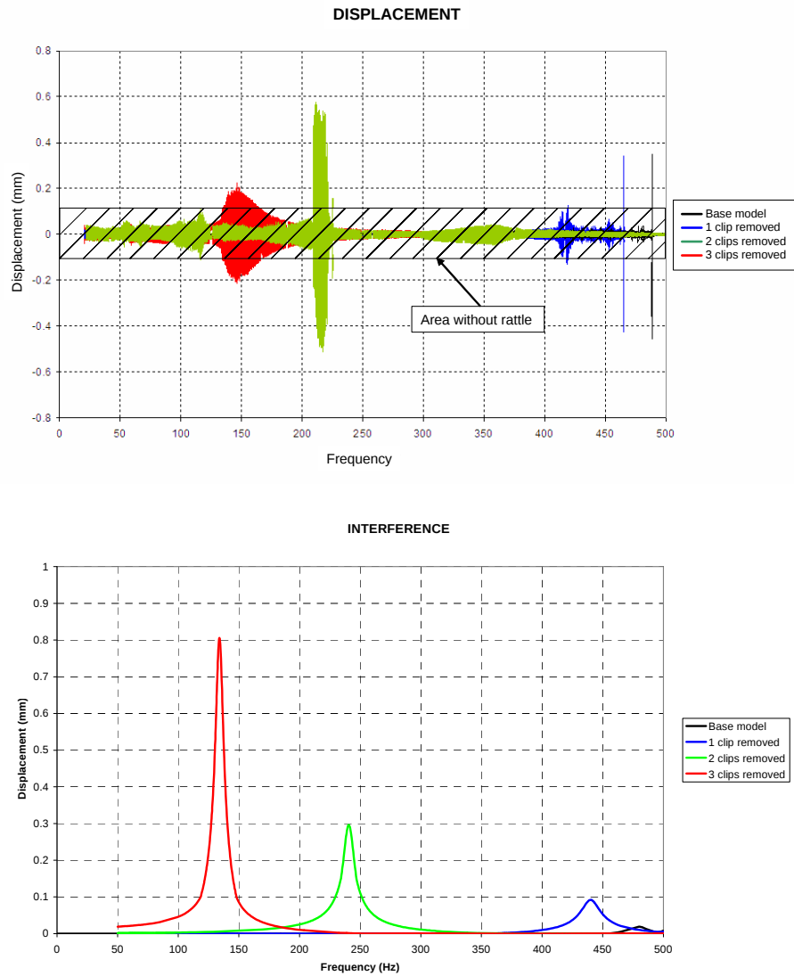
Figure 10. Top: Evolution of the rattle frequency with the elimination of clips in test (displacement). Bottom: Evolution of the rattle frequency with the elimination of clips in simulation (interference).
