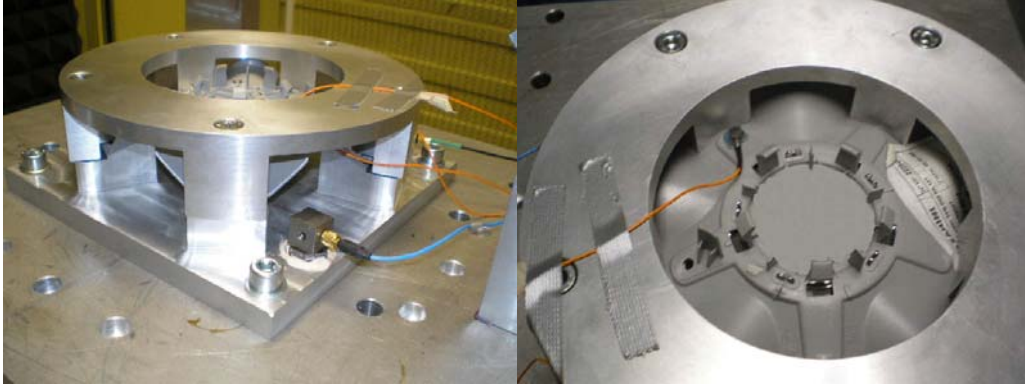
Figure 4. Testing tooling and detail of the clips
