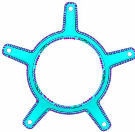
Figure 8. Sensor distribution at the inner ring
