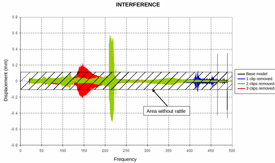
Figure 6. Evolution of the rattle frequency with the elimination of clips
