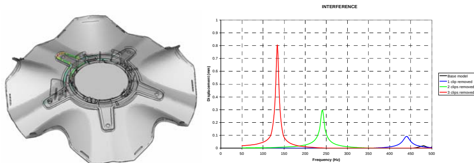
Figure 9. Left: visualization of the rattle results at an specific frequency. Right: frequency function that sums up the maximum penetration detected for the whole frequency range.
