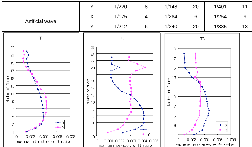
Figure 8 The curves of the maximum inter-story drift ratios under the action of the first group of natural wave
