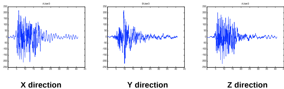
Figure 5 Artificial wave
