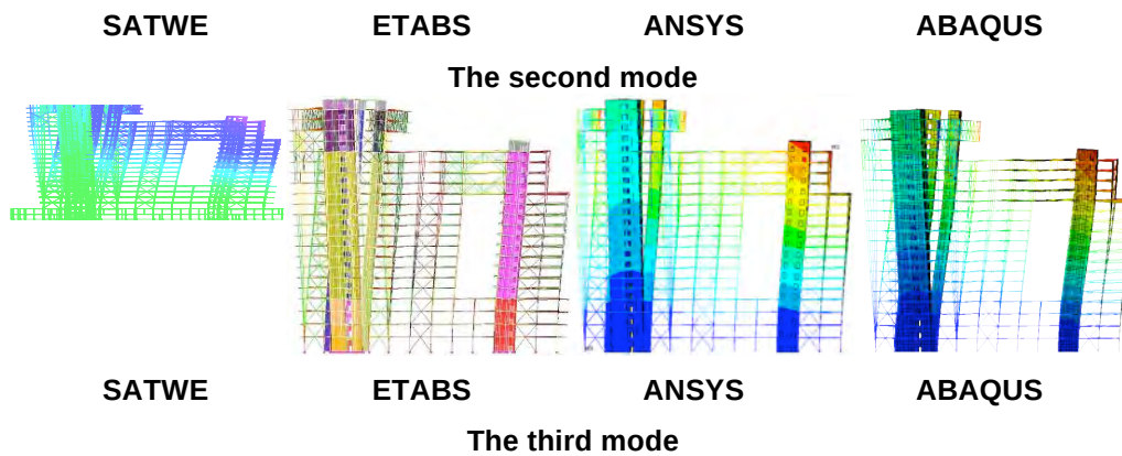
Figure 6 Vibration modes by different software
