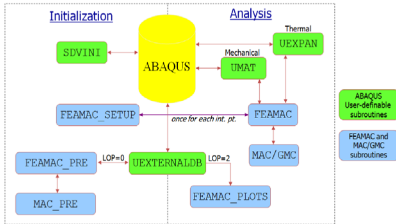
Figure 4 Schematic showing the implementation of the FEAMAC code within the Abaqus built-in UMAT framework.
