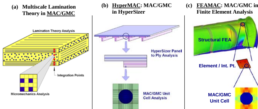
Figure 3. a) Multiscale lamination theory available in MAC/GMC. (b) HyperMAC coupling of HyperSizer with MAC/GMC. (c) FEAMAC coupling of MAC/GMC with finite element analysis.
