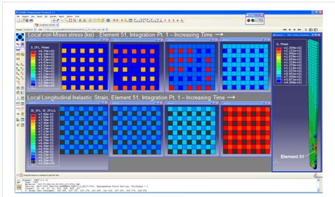
Figure 16. Shows the local von Mises stress and Inelastic strain within the RUC associated with integration point 1 of element 51 within the dogbone specimen. Global stress-strain response is that shown in Fig. 15 for the shear lag effective length case.
