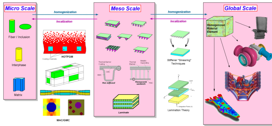
Figure 1. Illustration of associated levels scales for composite analysis.
