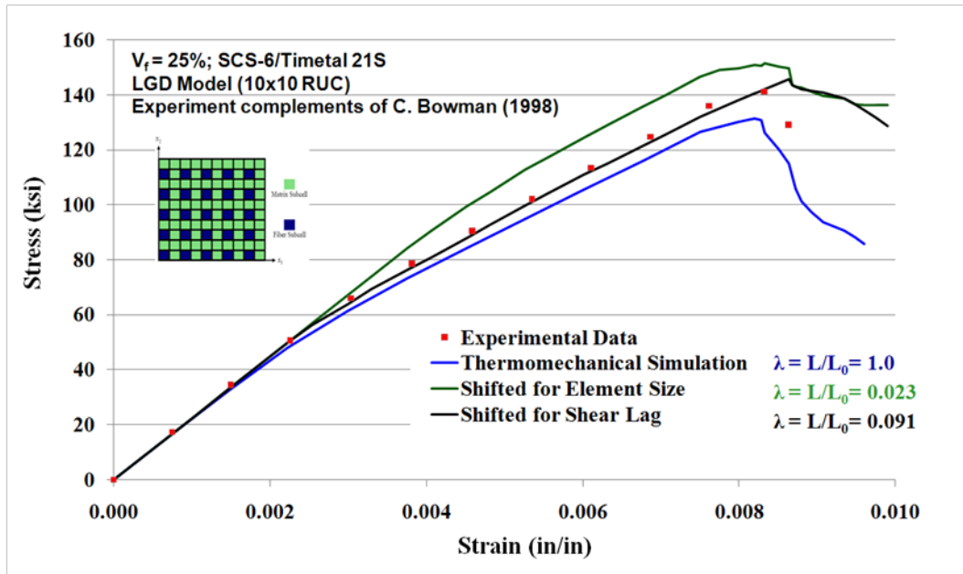
Figure 15. Comparison between experimental data and the local and global fiber strength distribution model prediction for a uniaxial longitudinal tension experiment of SiC/Ti (SCS-6/Ti-21S) at 650 °C wherein the residual stresses developed during heat treatment are accounted for.
