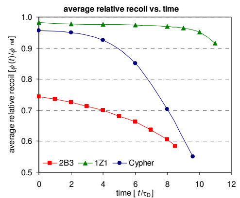
Fig. 2: Degradation of the 1Z1 stent [13, 14]. This design is much stiffer than the 2B3 and much of the deformation and degradation is confined to the junction points and sharp crowns of the stent rings. If failure occurs at these locations, struts that are mostly non-degraded can provoke embolic complications downstream. As the material loses its integrity, buckling of the cylindrical structure is observed to initiate [12].
