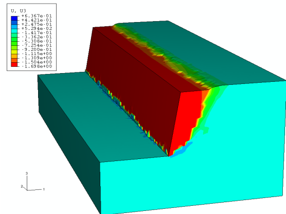
Figure 16: Vertical displacement at an intermediate post-failure instant for the model analyzed using Abaqus/Explicit
