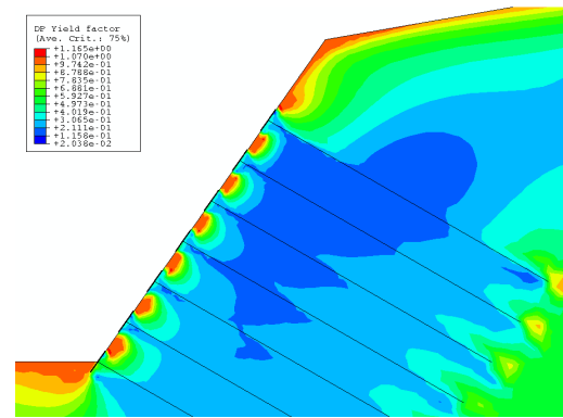
Figure 15: DP Yield Factor for the seven nail case
