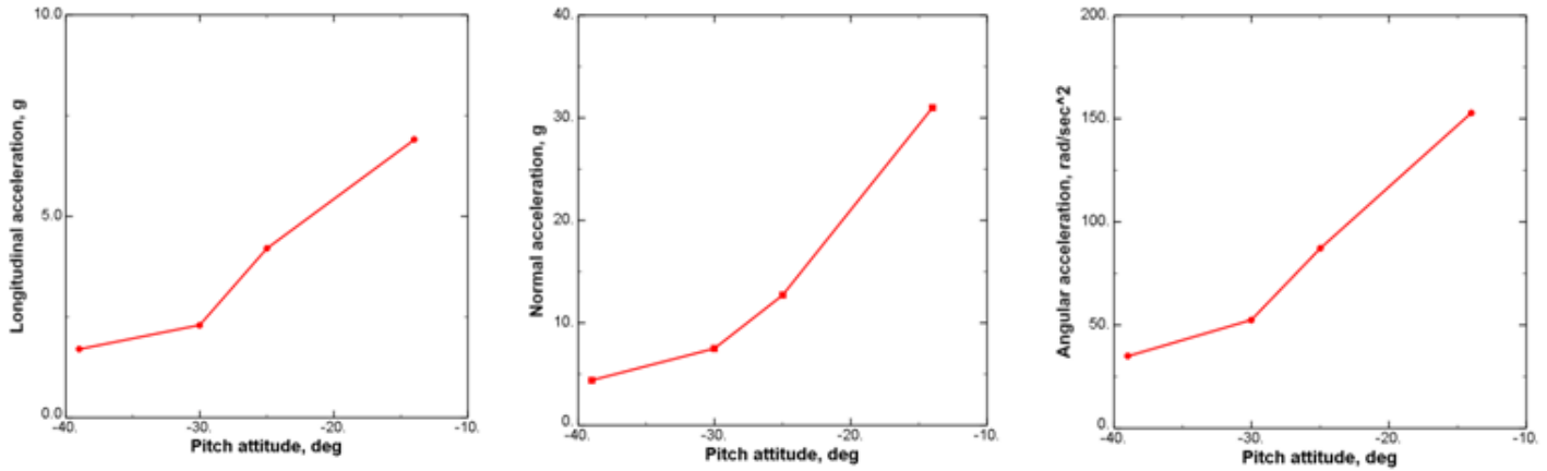
Figure 5: Peak longitudinal, normal and angular accelerations versus vehicle pitch
