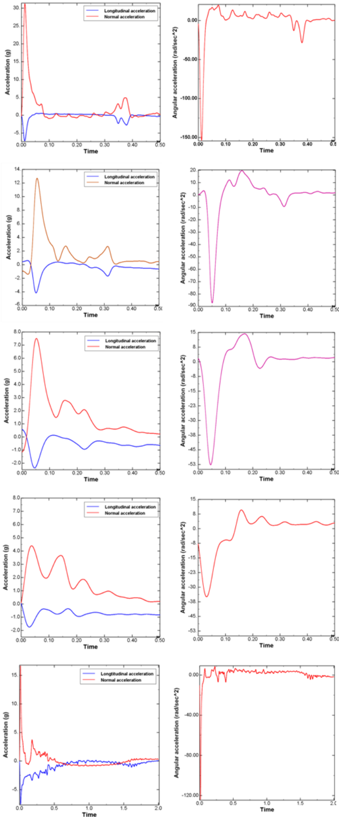
Figure 3: Longitudinal, normal and angular accelerations of the re-entry vehicle for Cases 1, 2, 3, 4, & 5
