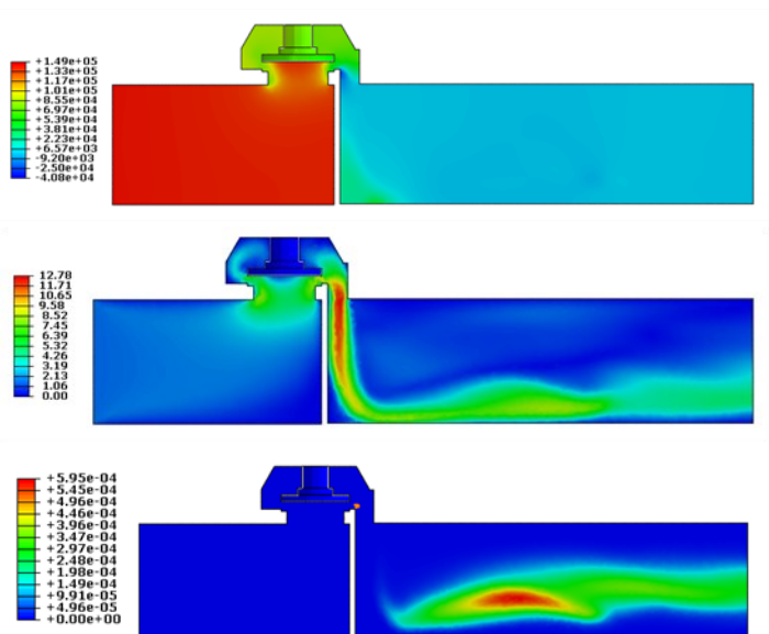
Figure 13: Fluid pressure (top), velocity (middle), and kinematic turbulent viscosity (bottom) at mean plunger displacement
