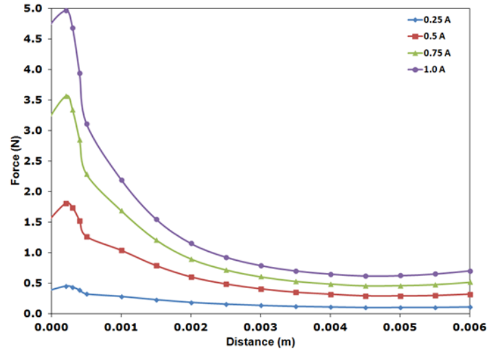
Figure 6: Calculated force versus plunger displacement for various values of electric current
