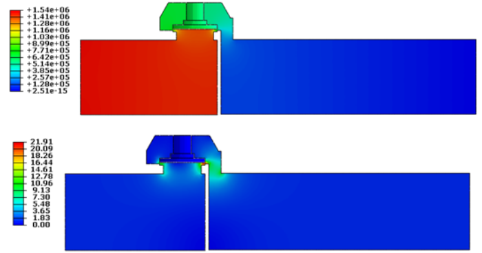
Figure 12: Fluid pressure (top) and velocity (bottom) at t = 0
