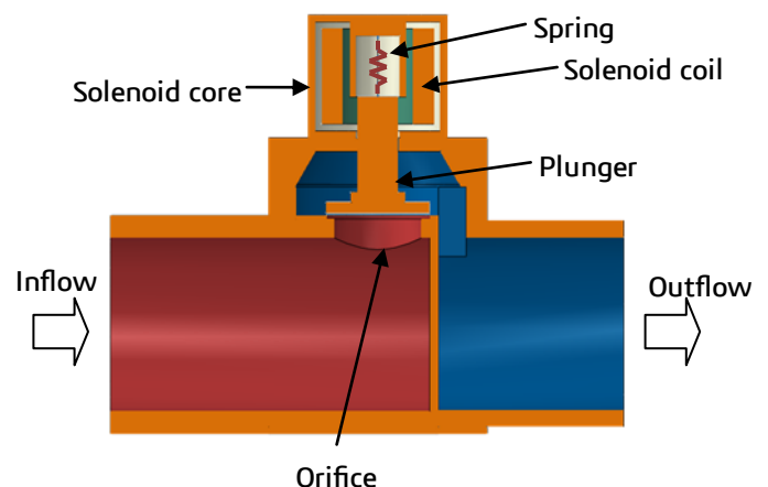
Figure 1: Schematic diagram of the solenoid valve model
