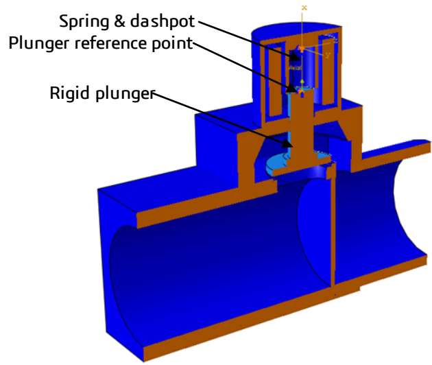
Figure 8: Schematic diagram of structural model (view-cut through the symmetry plane)
