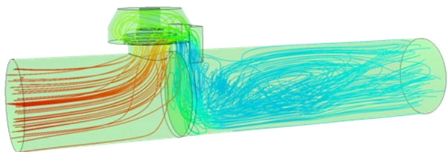
Figure 14: Streamlines colored by pressure at mean plunger displacement
