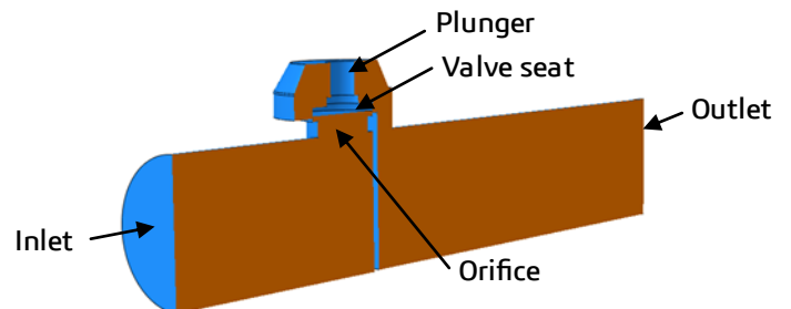
Figure 7: Schematic diagram of CFD model (view-cut through the symmetry plane)
