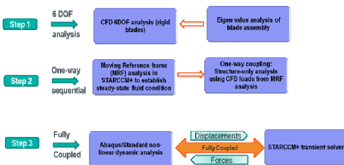
Figure 3: Three-step simulation workflow
