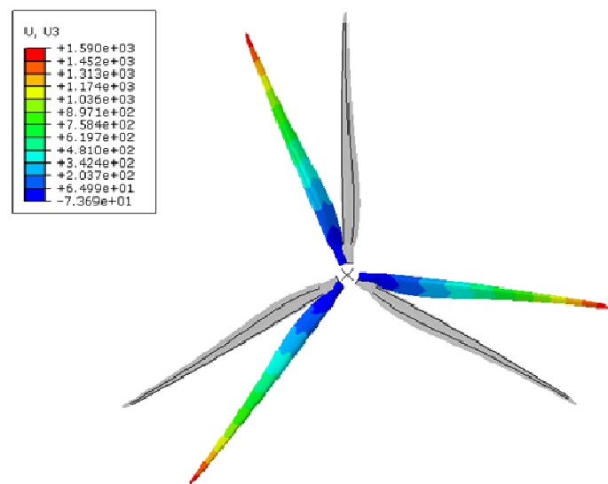
Figure 5: Bending deflection (mm), sequentially coupled FSI analysis
