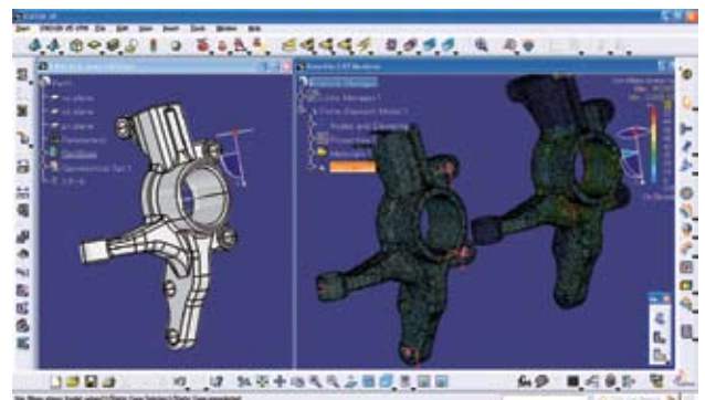
Structural analysis of a steering knuckle including virtual rigid parts
