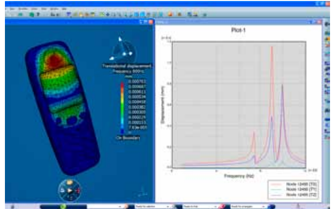
The dynamic harmonic response of a phone subjects to the speaker vibration can be determined easily.
