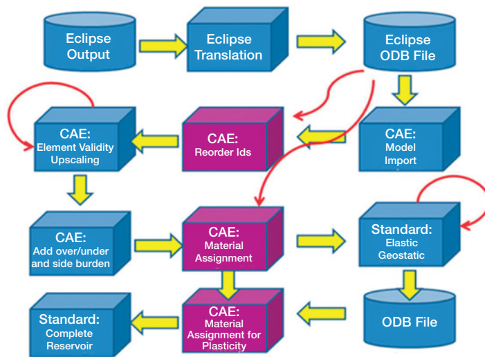
Figure 3. Reservoir geomechanics workflow. An output database file (ODB) is created from ECLIPSE and imported into Abaqus/CAE for creation of an FEA geomechanical model from which the stress distribution over a reservoir can be derived. A plastic analysis then predicts the geomechanical deformations (subsidence) in the surrounding terrain that will result from this stress.
