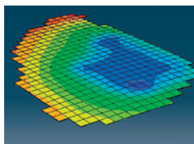
Figure 2. (Left) Active region generated from the flow simulation solution. (Bottom) Abaqus mesh showing the active region within a reservoir. Linking ECLIPSE with Abaqus incorporates the geomechanical effects of extraction for a more realistic simulation of full-site development over time.
