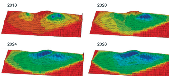
Figure 4. Four increments in an Abaqus FEA simulation of subsidence in a hypothetical oilfield, displayed over ten years. Blue areas denote greatest downward displacement of the surface. This particular example from Eni contains just 300,000 degrees of freedom; enhancements in model setup and automation now allow the running of huge full-scale models with millions of DOF in just a few hours. Rock faults (not pictured here) can be included in simulations.
